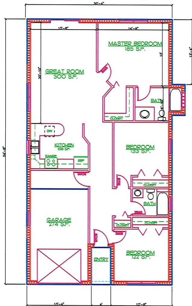
FLOOR PLAN 1/4"=1'-0"
